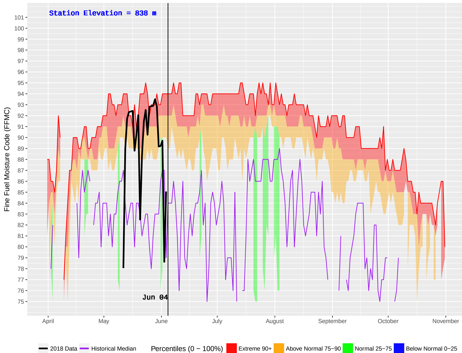
HOWARD (343) : Historical (1970–2016) and Current (2018) Noon Fine Fuel Moisture Code (FFMC)
