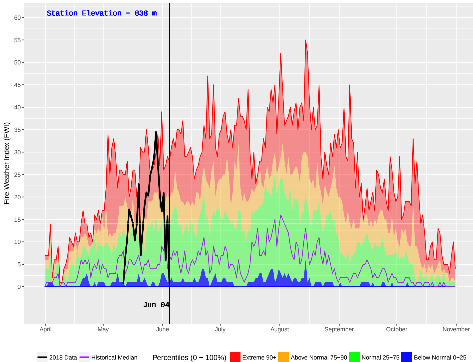
HOWARD (343) : Historical (1970–2016) and Current (2018) Noon Fire Weather Index (FWI)
