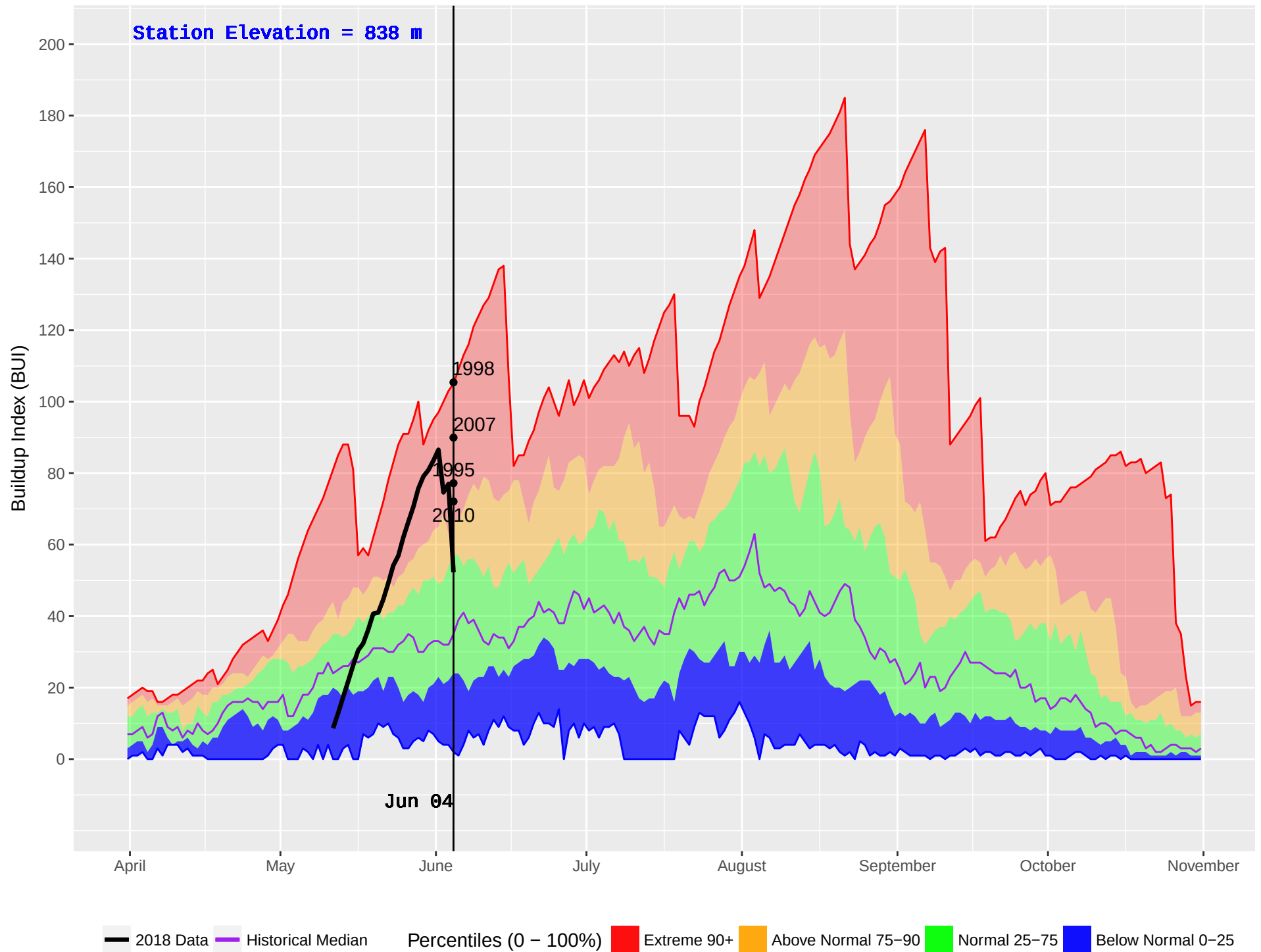
HOWARD (343) : Historical (1970–2016) and Current (2018) Noon Buildup Index (BUI)
